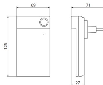
Repeater Modul Danfoss Icon™
