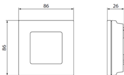
Wireless Raumthermostat Danfoss Icon™
