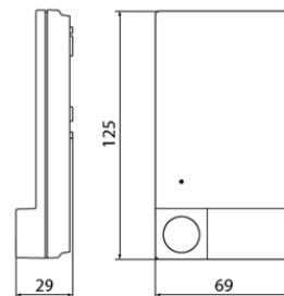
Funk Modul Danfoss Icon™
